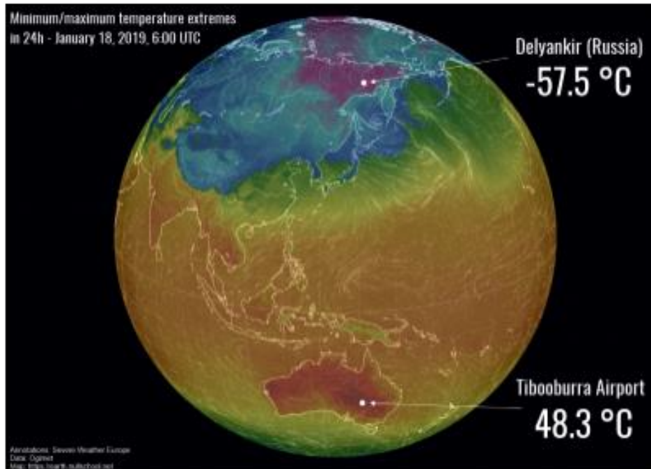
Map Earthwindmap
