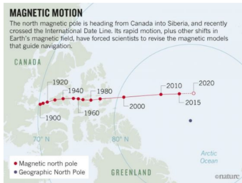
The north magnetic pole moves from Canada to Siberia
