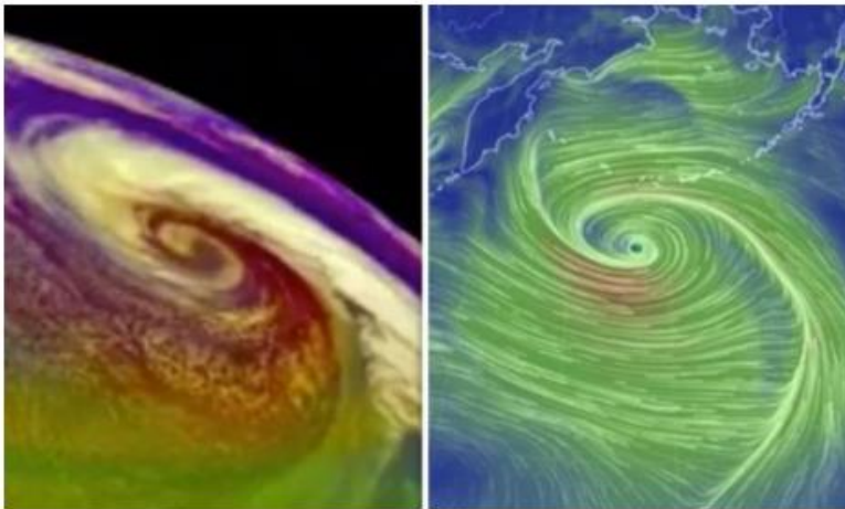
Double bombogenesis hits off the Aleutian islands in Alaska on January 10, 2019
