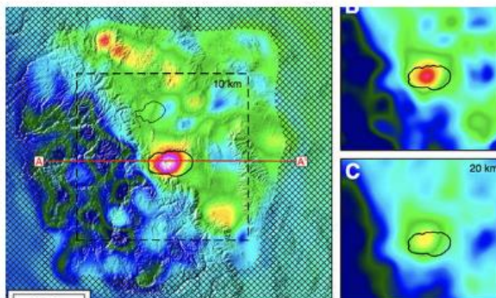
A thermal image of the Long Valley Caldera shows huge amount of magma concentrating under the supervolcano. GSA
