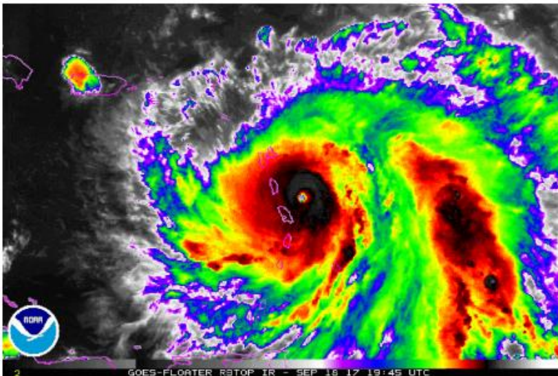
Infrared satellite loop of Maria making landfall in Dominica on September 19, 2017. Just before devastating Puerto Rico.
