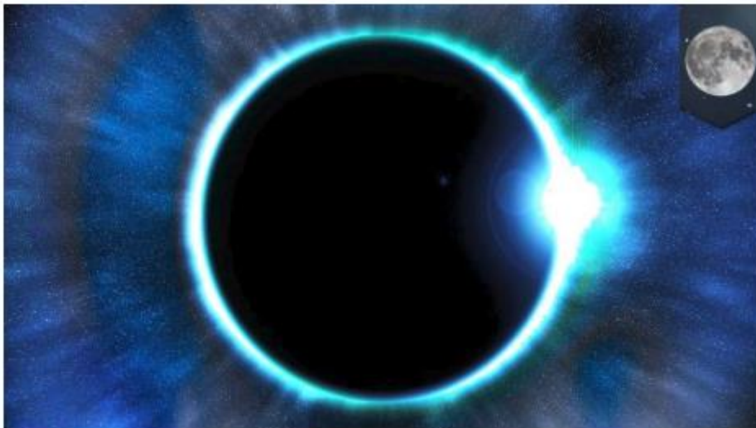
Jan 31: Super Blue Moon Eclipse: It's not just a lunar eclipse, or a Blue Moon, or a supermoon. It's all three!
