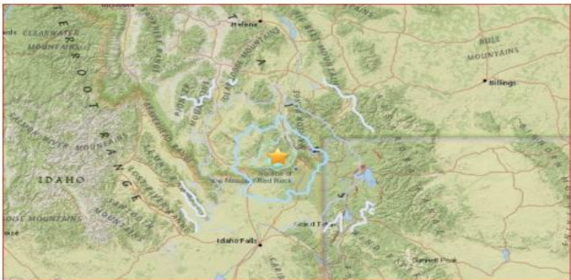
Location map of the unusual strong earthquake near West Yellowstone, Montana on June 13, 2016. Via USGS
