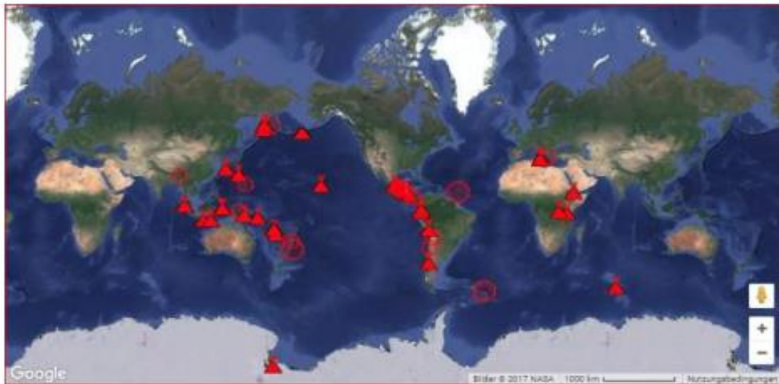
There are currently 32 volcanoes erupting around the world as of October 3, 2017. Circles represent earthquakes larger than M5.0 in the past 24 hours.
