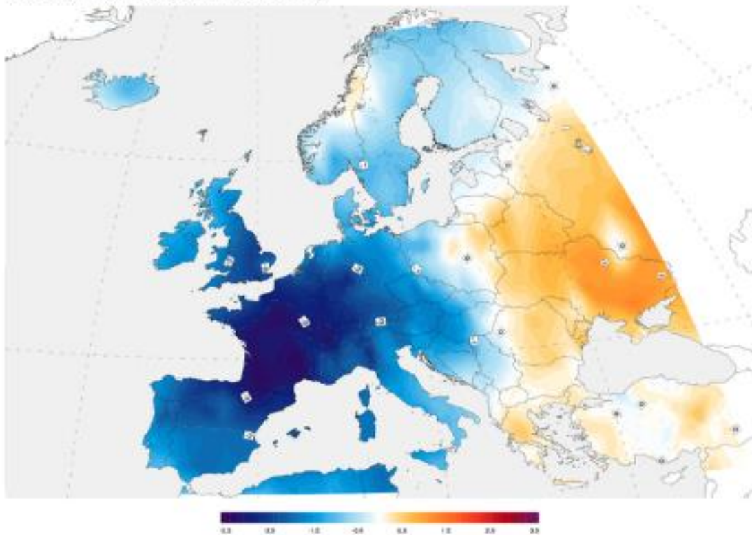
1816 Summer Temperature Anomaly
