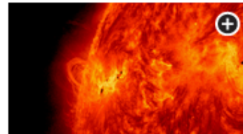
NASA's Solar Dynamics Observatory captured this image of the X1.2 class solar flare on May 14, 2013. (NASA/SDO)
